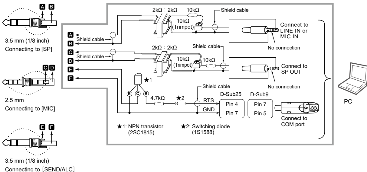
Interface circuit example for digital modes (User supplied)
