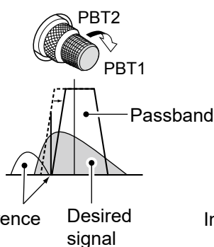
Cutting the lower passband
