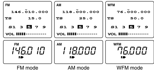
FM mode
