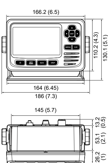
MA-510TR with the mounting bracket
