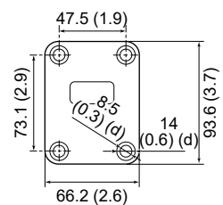
Base (Top view)
